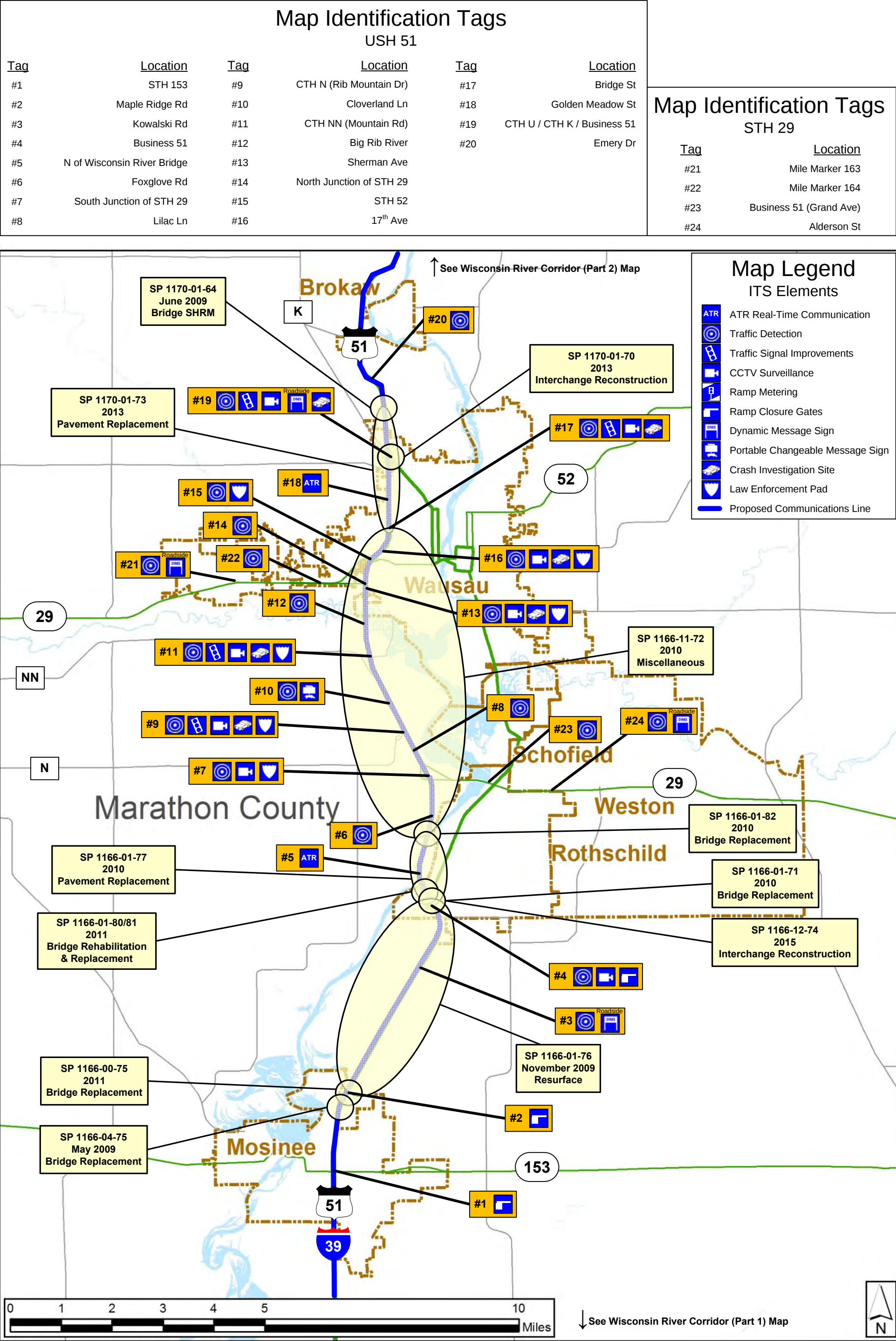
Wausau – TOIP Based ITS Deployment Figure 34
